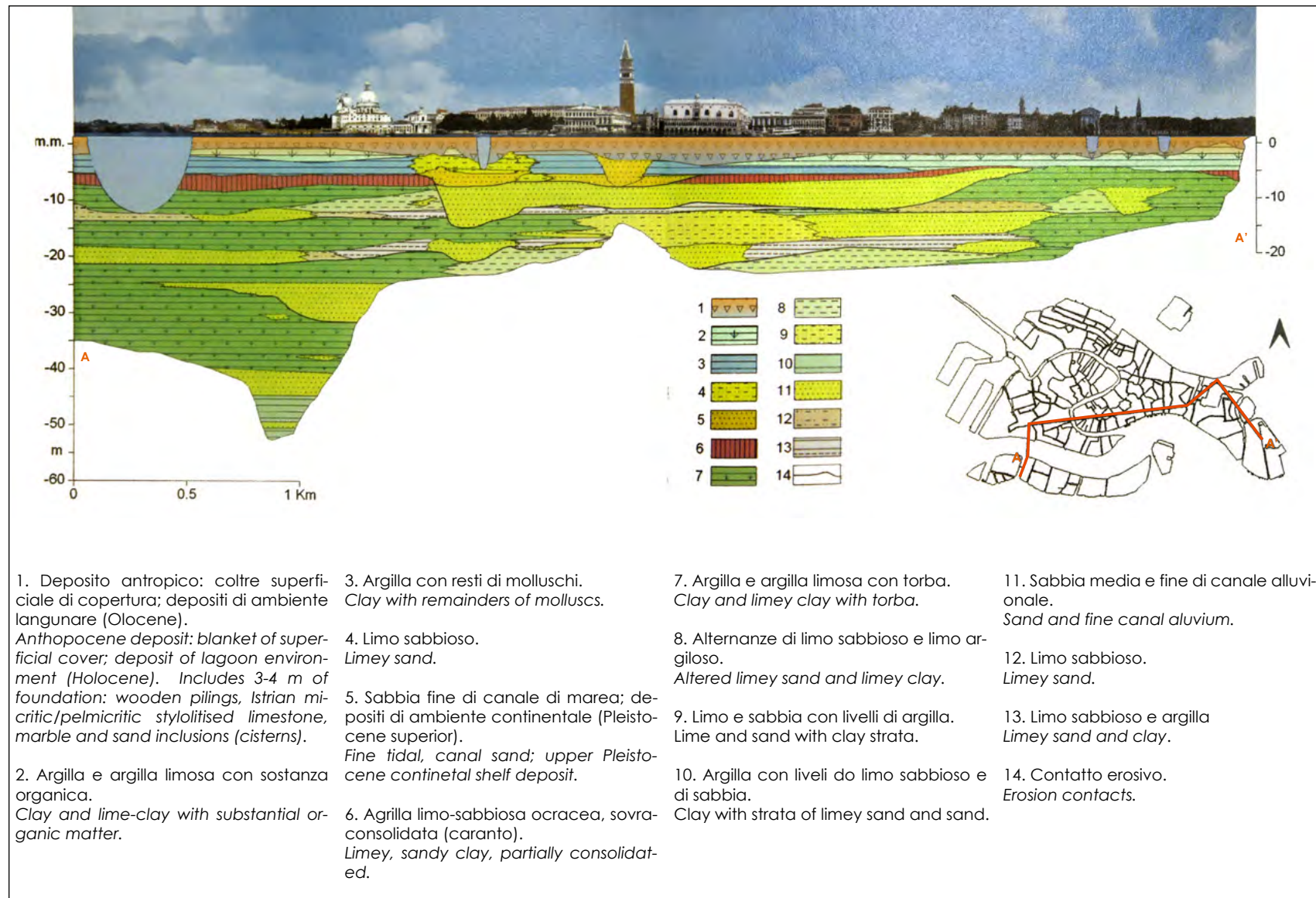
Fig. 6. Venice cross-section. Adapted from Zezza, Fulvio, Venezia citta d'acqua , Marsilio Edition, 2014. Translation of legend by artist.
